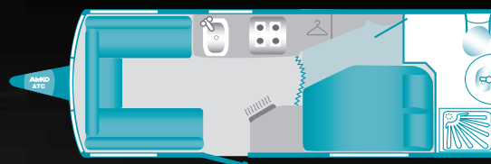
624 - 4 Berth (TWIN AXLE)
